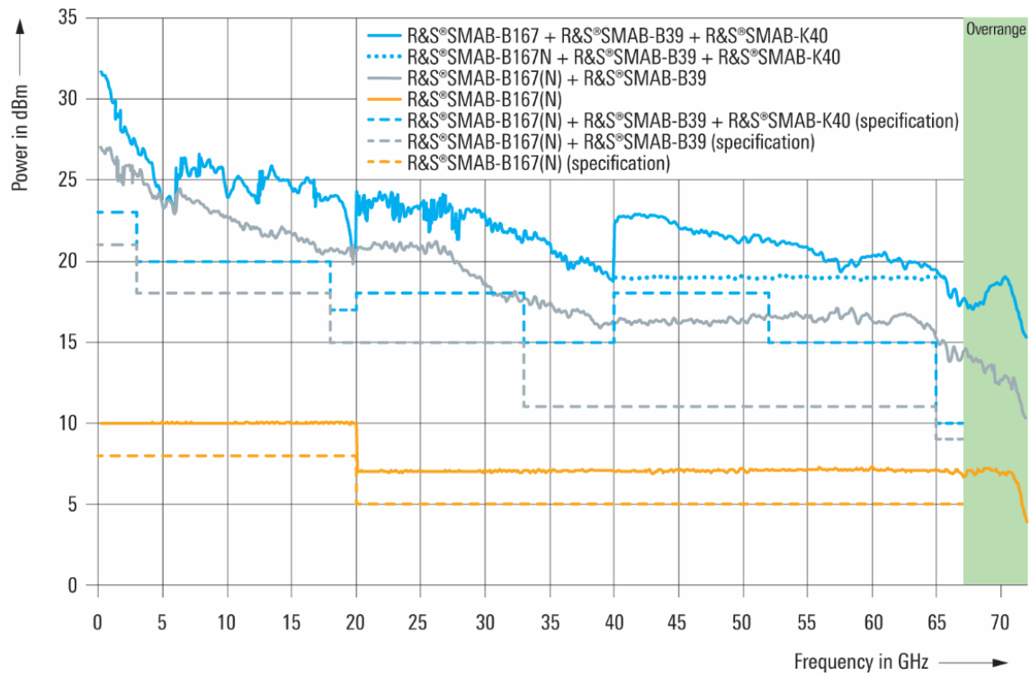
Specified and measured maximum available output power versus frequency
