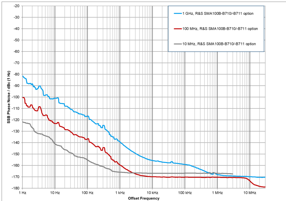
Measured SSB phase noise of reference outputs at f = 10 MHz, 100 MHz and 1 GHz with the R&S®SMAB-B710(N) and R&S®SMAB-B711(N) options ( f = 100 MHz and 1 GHz only available with the R&S®SMAB-K703 option)
