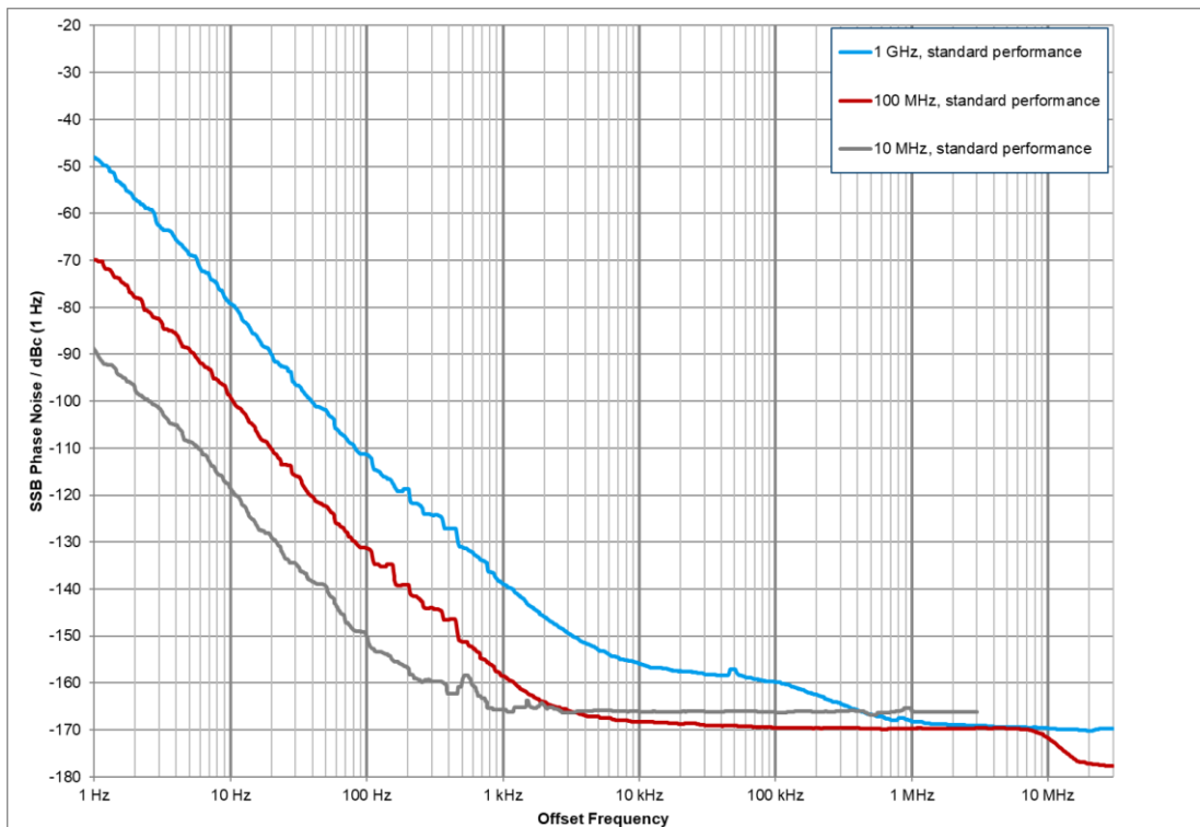
Measured SSB phase noise of reference outputs at f = 10 MHz, 100 MHz and 1 GHz ( f = 100 MHz and 1 GHz only available with the R&S®SMAB-K703 option)
